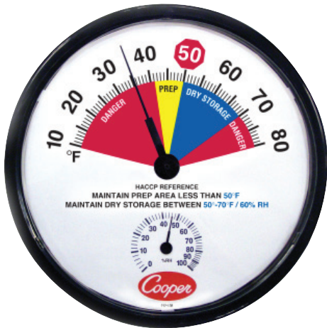
212-158 Prep Area and Dry Storage Thermometer Consolidates from two units to one replacing the 212-154 and 212-155.
