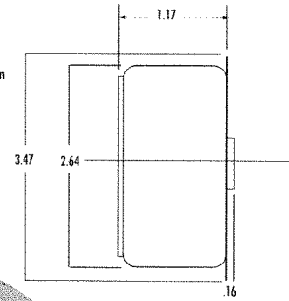
Mounting Dimensions DM120S/DM450S
