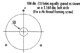
Mounting Dimensions DM120S/DM450S
