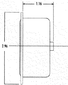
Mounting Dimensions DM120/DM450
